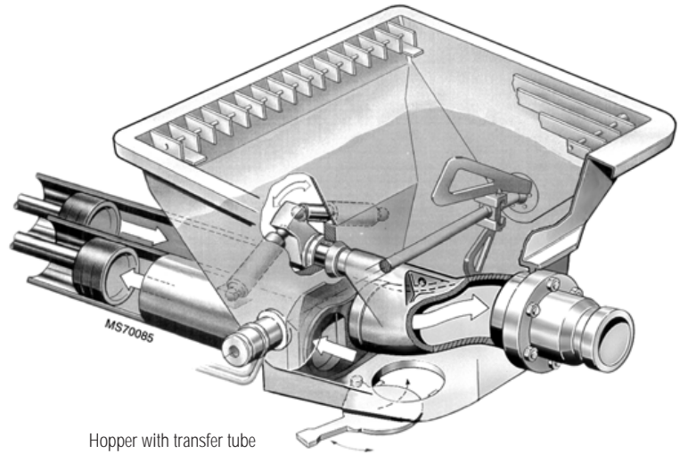
Hopper with transfer tube
